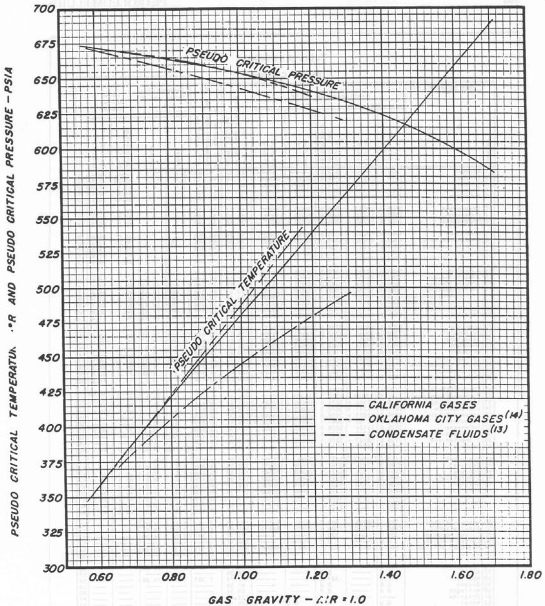
Figure 17—Pseudo-critical Constants of Gases and Condensate Well Fluids
