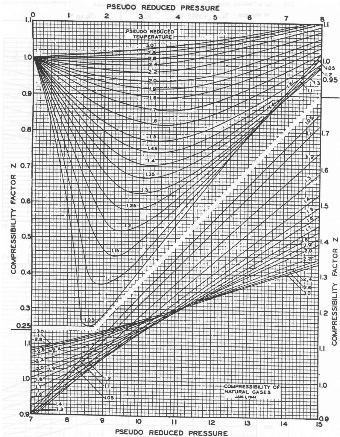
Figure 15—Compressibility Factors for Natural Gases (After Standing and Katz, Trans. AIME, 1942)
