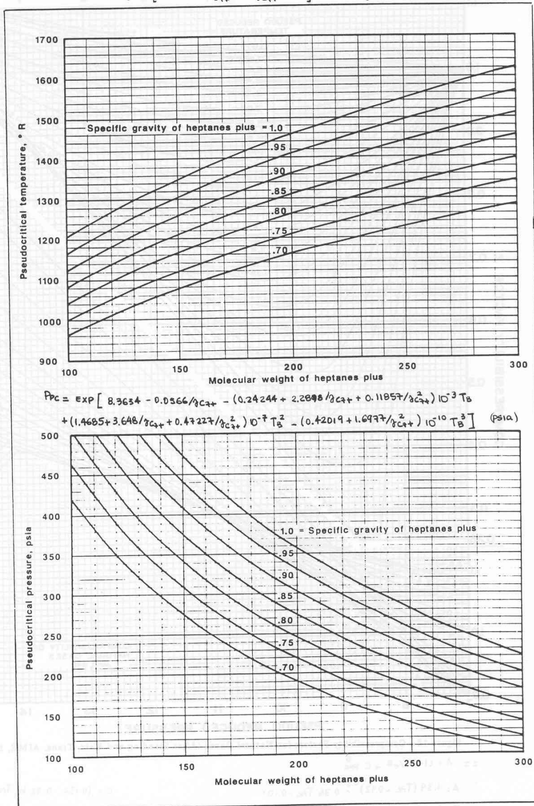
Fig. 3-10. Pseudocritical properties of heptanes plus.
